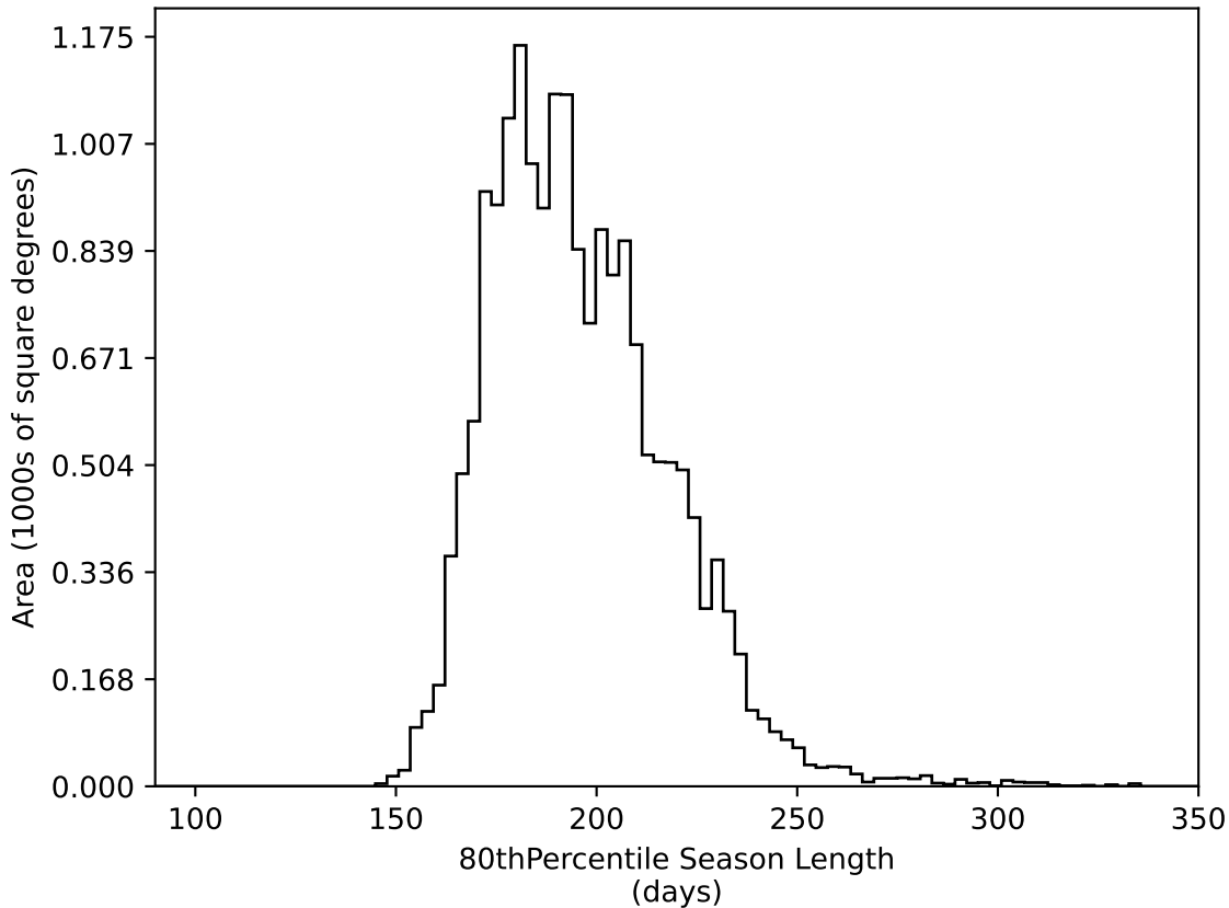
ddf_loaded_fl4_v3.4_10yrs WFD all bands: 80thPercentile Season Length
