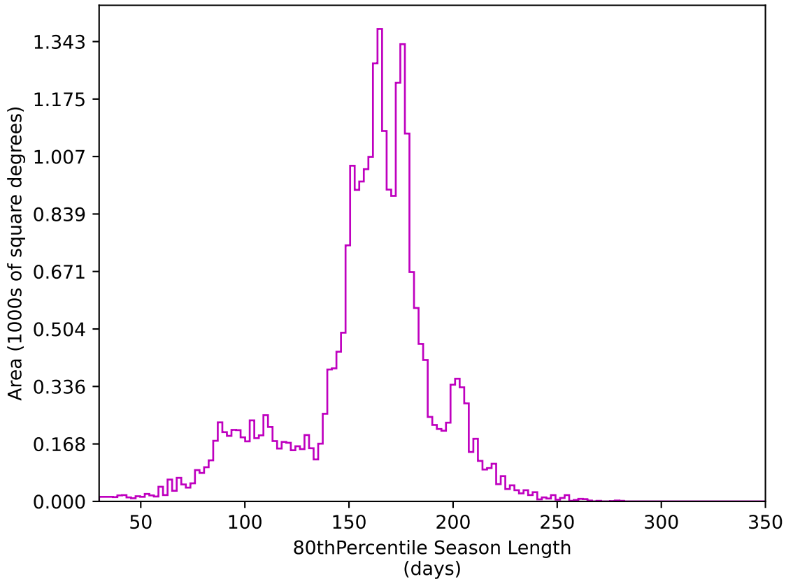
ddf_loaded_fl4_v3.4_10yrs All sky z band: 80thPercentile Season Length
