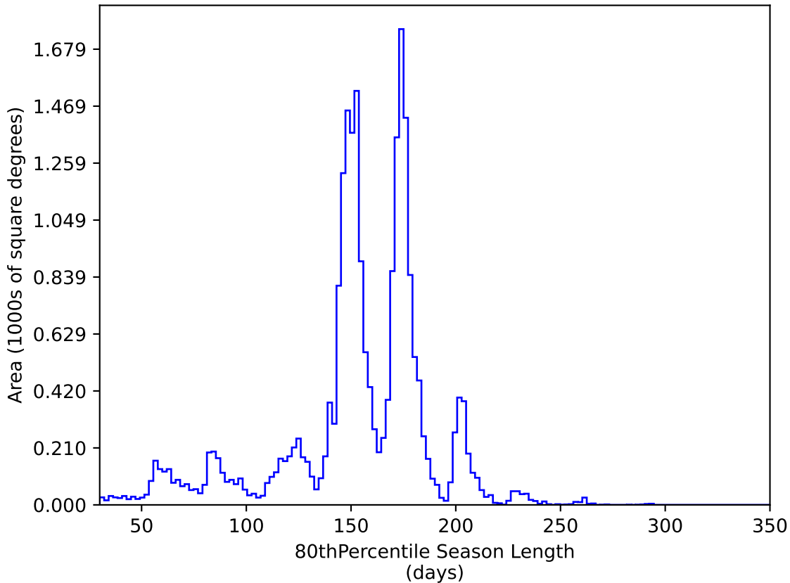
ddf_loaded_fl4_v3.4_10yrs All sky y band: 80thPercentile Season Length
