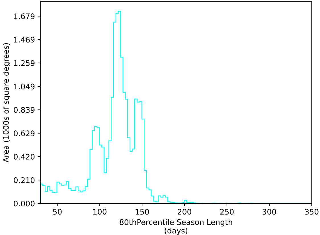
ddf_loaded_fl4_v3.4_10yrs All sky u band: 80thPercentile Season Length
