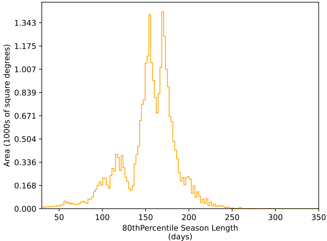
ddf_loaded_fl4_v3.4_10yrs All sky r band: 80thPercentile Season Length
