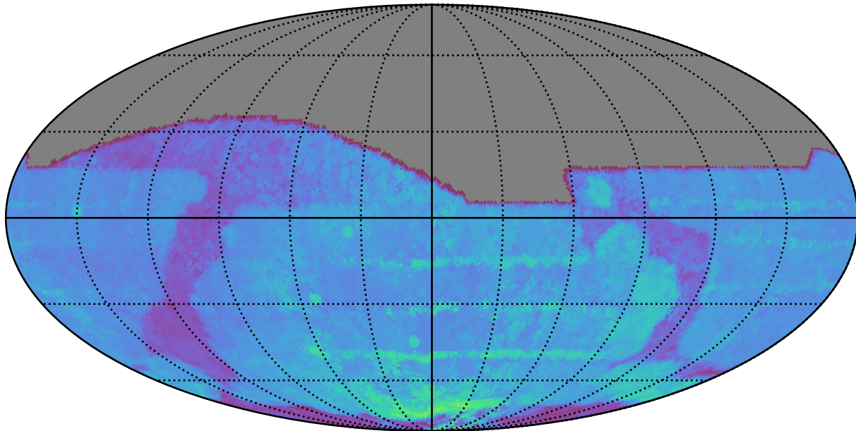
ddf_loaded_fl4_v3.4_10yrs All sky i band: 80thPercentile Season Length
