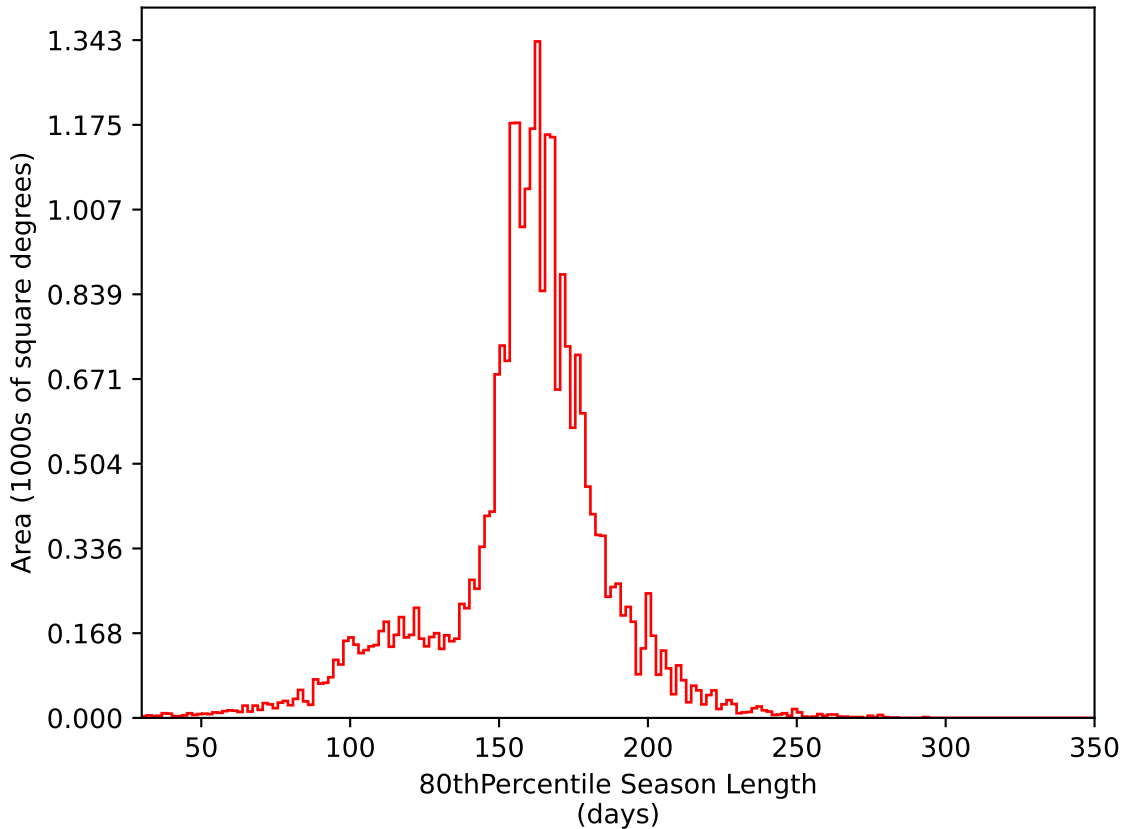
ddf_loaded_fl4_v3.4_10yrs All sky i band: 80thPercentile Season Length
