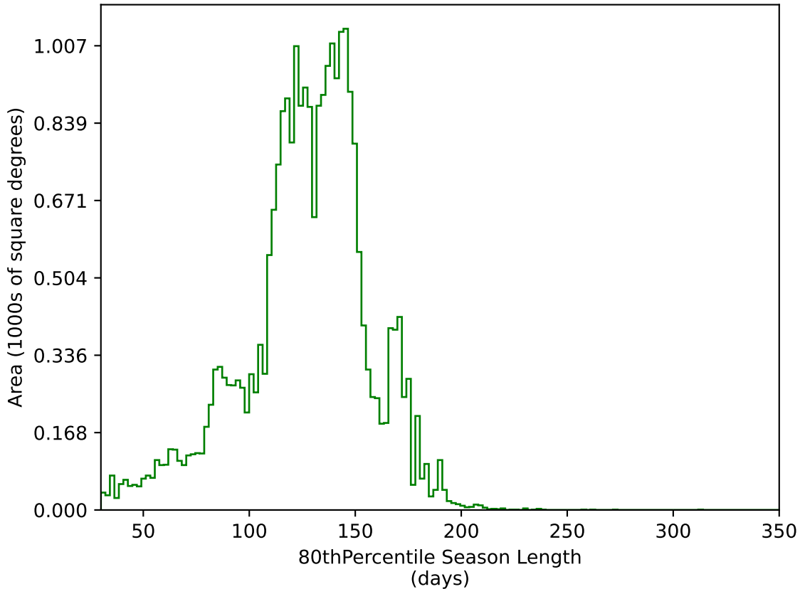
ddf_loaded_fl4_v3.4_10yrs All sky g band: 80thPercentile Season Length
