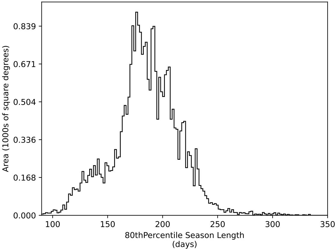
ddf_loaded_fl4_v3.4_10yrs All sky all bands: 80thPercentile Season Length
