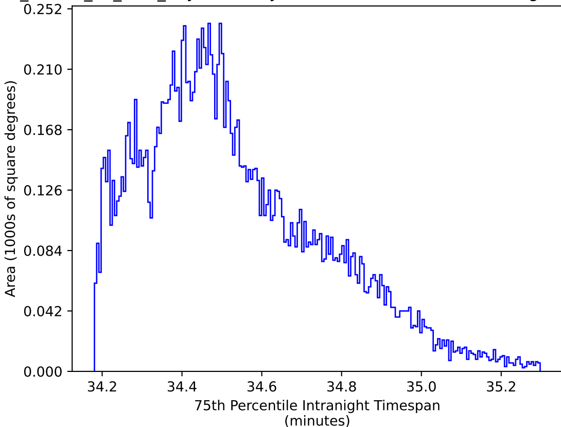
ddf_loaded_fl4_v3.4_10yrs WFD zy bands: 75th Percentile Intranight Timespan
