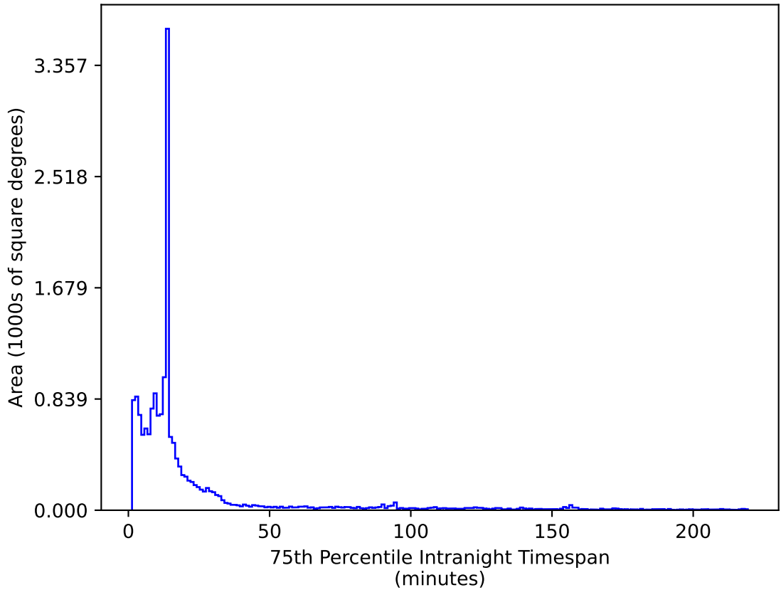
ddf_loaded_fl4_v3.4_10yrs WFD z band: 75th Percentile Intranight Timespan
