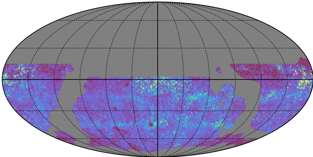
ddf_loaded_fl4_v3.4_10yrs WFD y band: 75th Percentile Intranight Timespan
