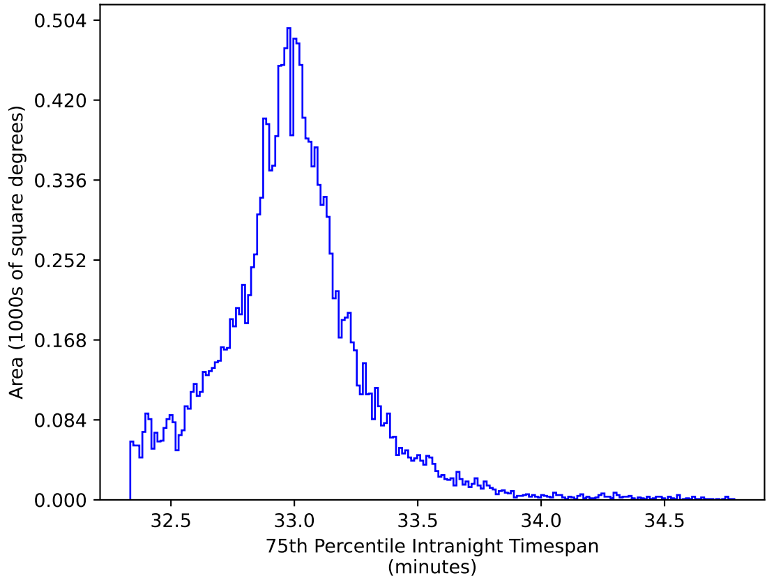
ddf_loaded_fl4_v3.4_10yrs WFD y band: 75th Percentile Intranight Timespan
