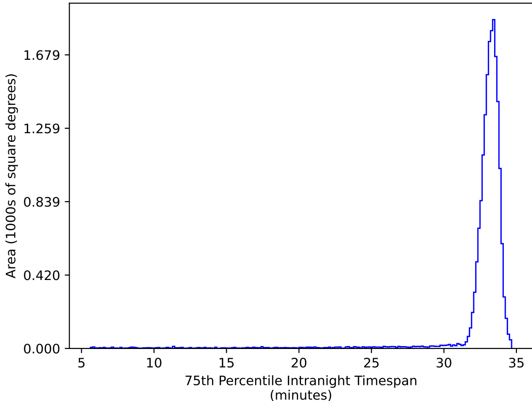
ddf_loaded_fl4_v3.4_10yrs WFD ug bands: 75th Percentile Intranight Timespan
