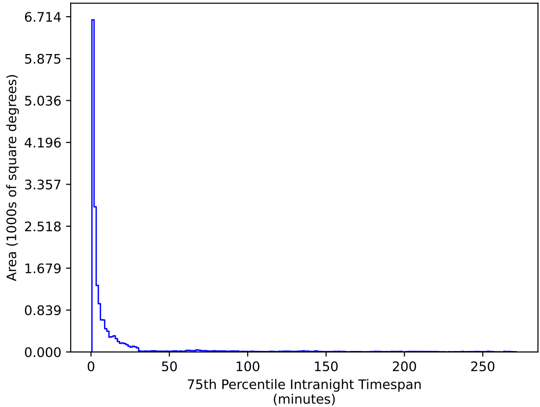
ddf_loaded_fl4_v3.4_10yrs WFD u band: 75th Percentile Intranight Timespan
