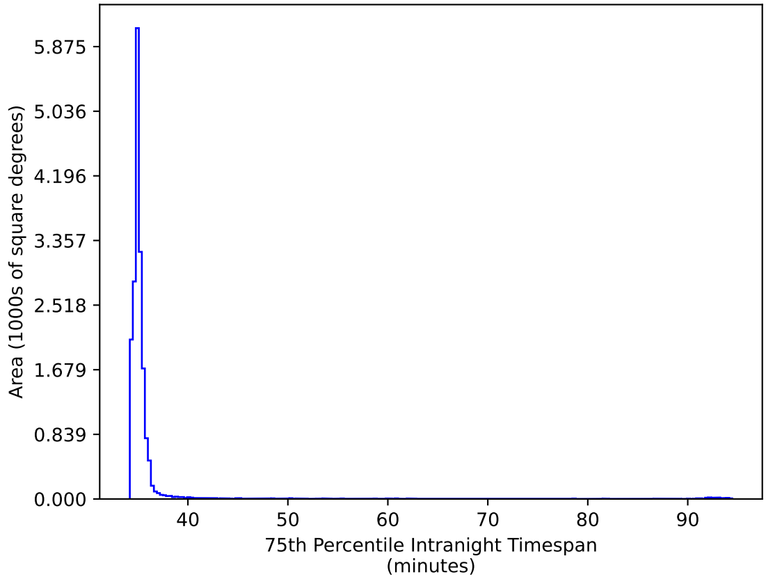
ddf_loaded_fl4_v3.4_10yrs WFD ri bands: 75th Percentile Intranight Timespan
