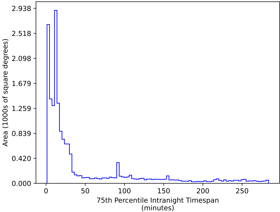
ddf_loaded_fl4_v3.4_10yrs WFD r band: 75th Percentile Intranight Timespan
