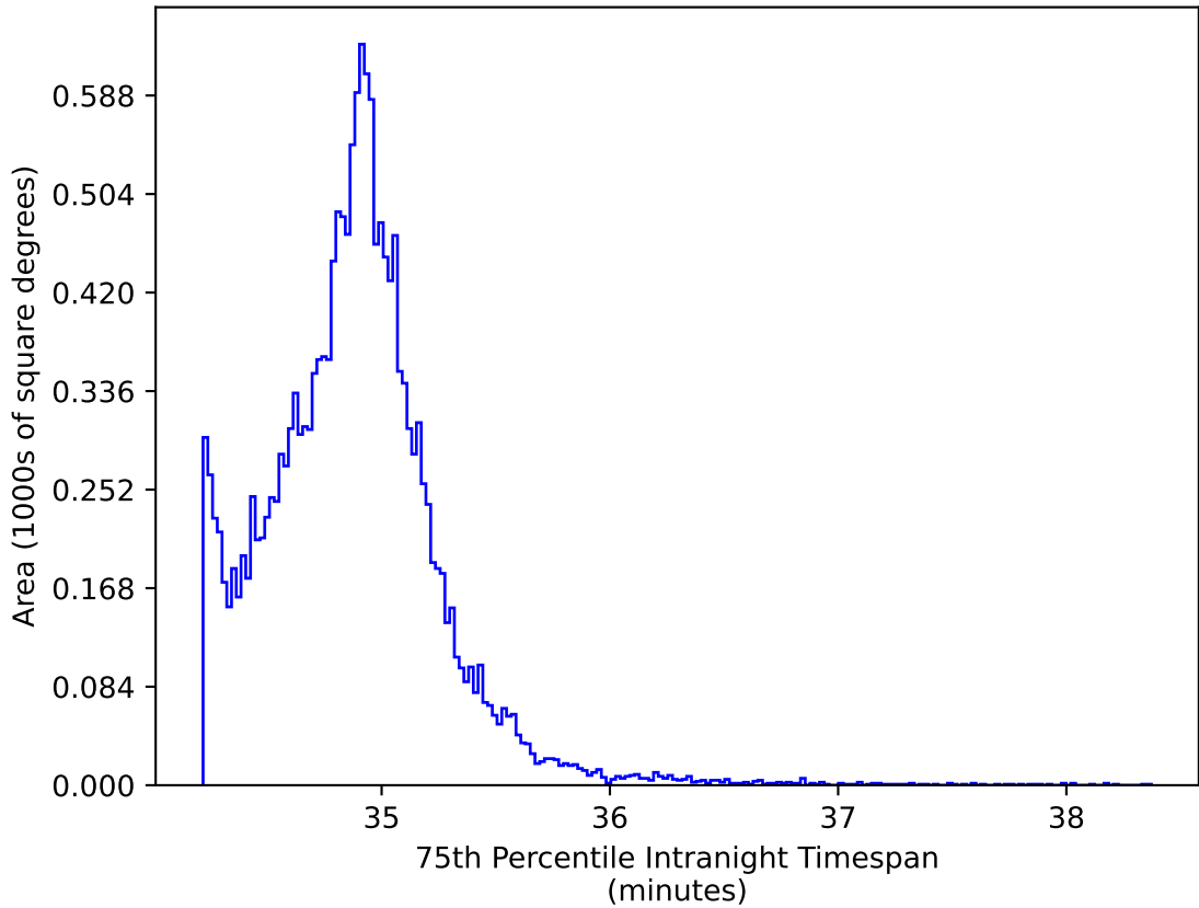
ddf_loaded_fl4_v3.4_10yrs WFD iz bands: 75th Percentile Intranight Timespan
