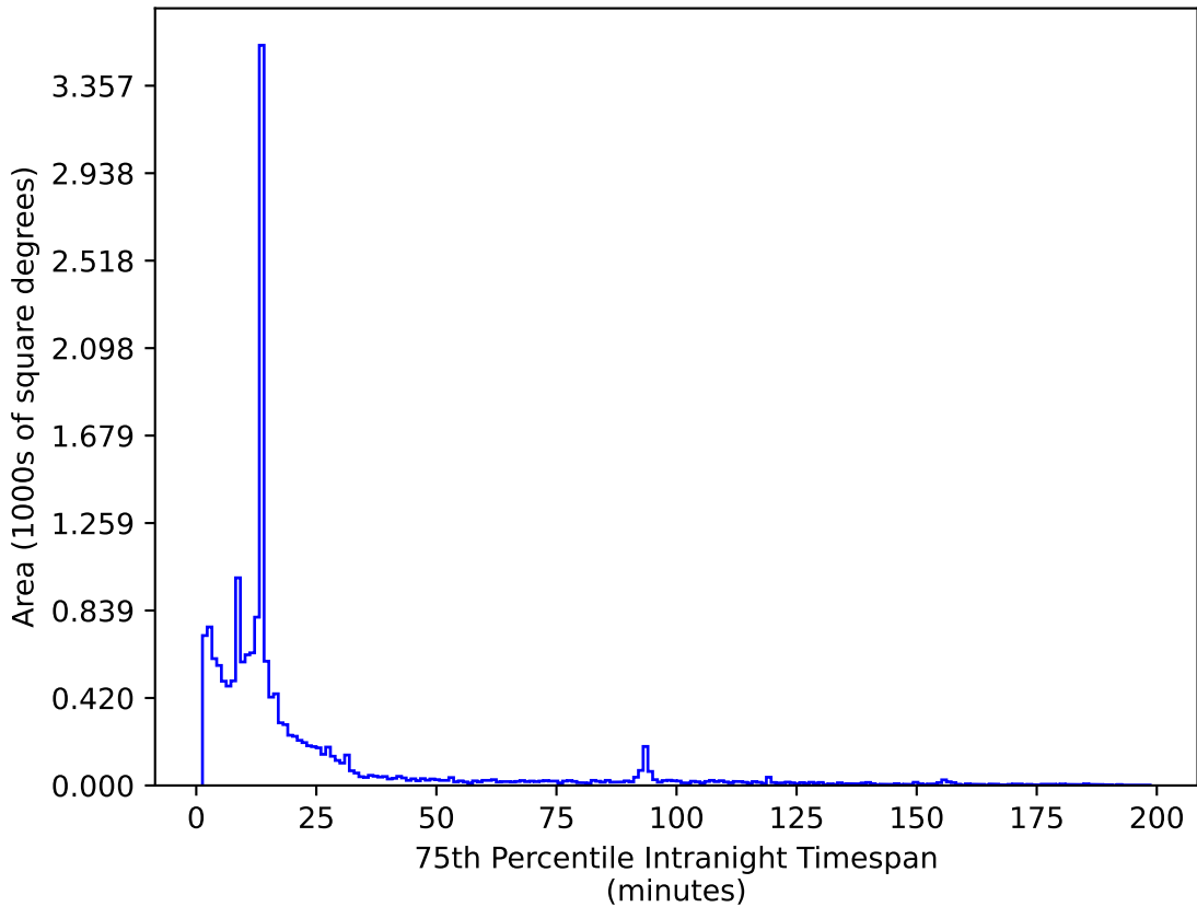
ddf_loaded_fl4_v3.4_10yrs WFD i band: 75th Percentile Intranight Timespan
