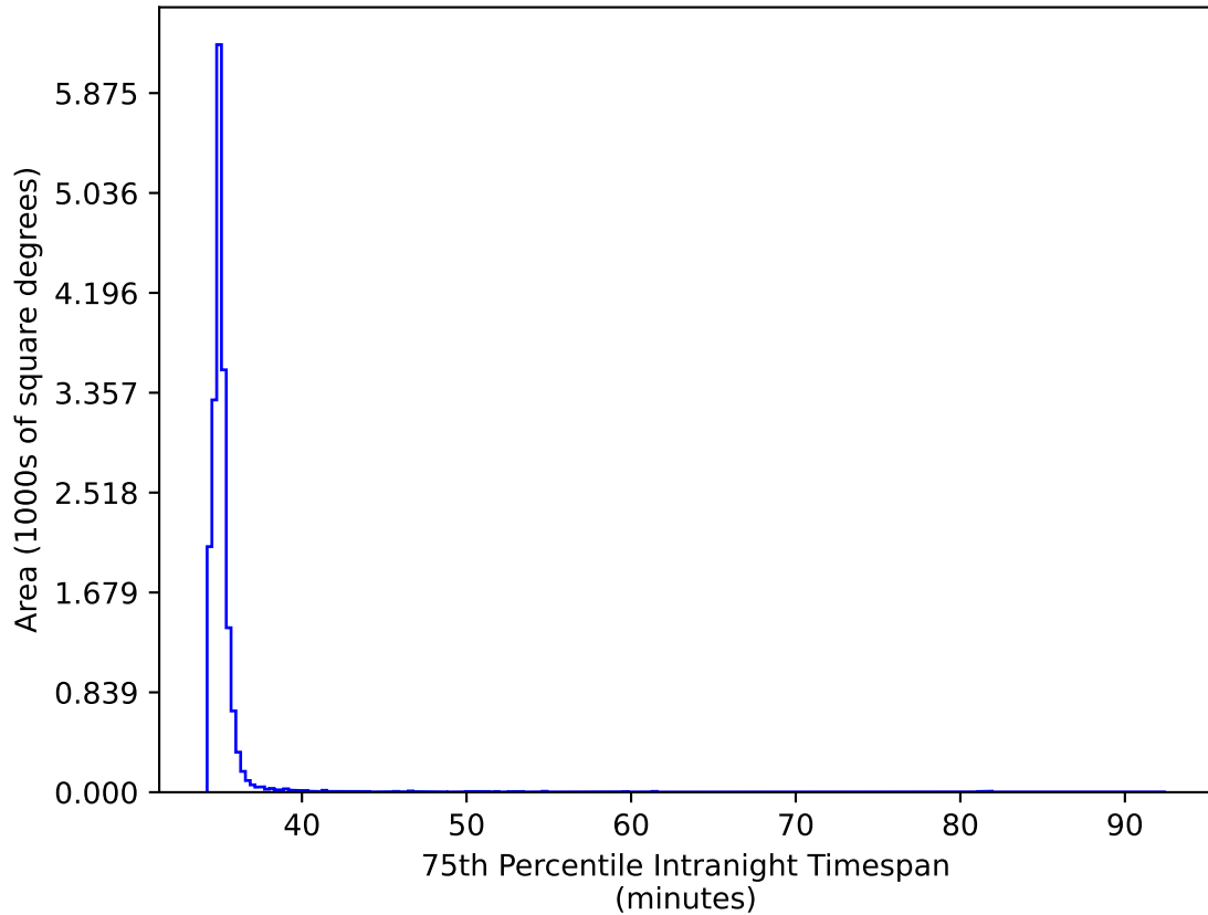
ddf_loaded_fl4_v3.4_10yrs WFD gr bands: 75th Percentile Intranight Timespan
