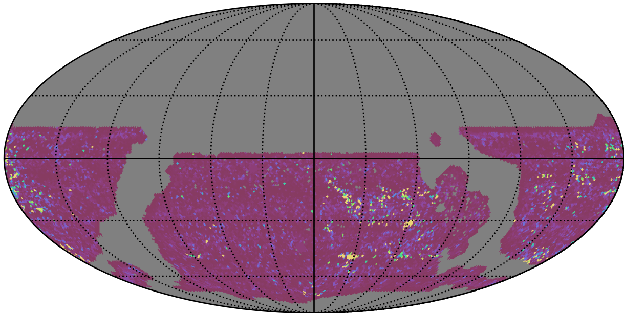
ddf_loaded_fl4_v3.4_10yrs WFD g band: 75th Percentile Intranight Timespan
