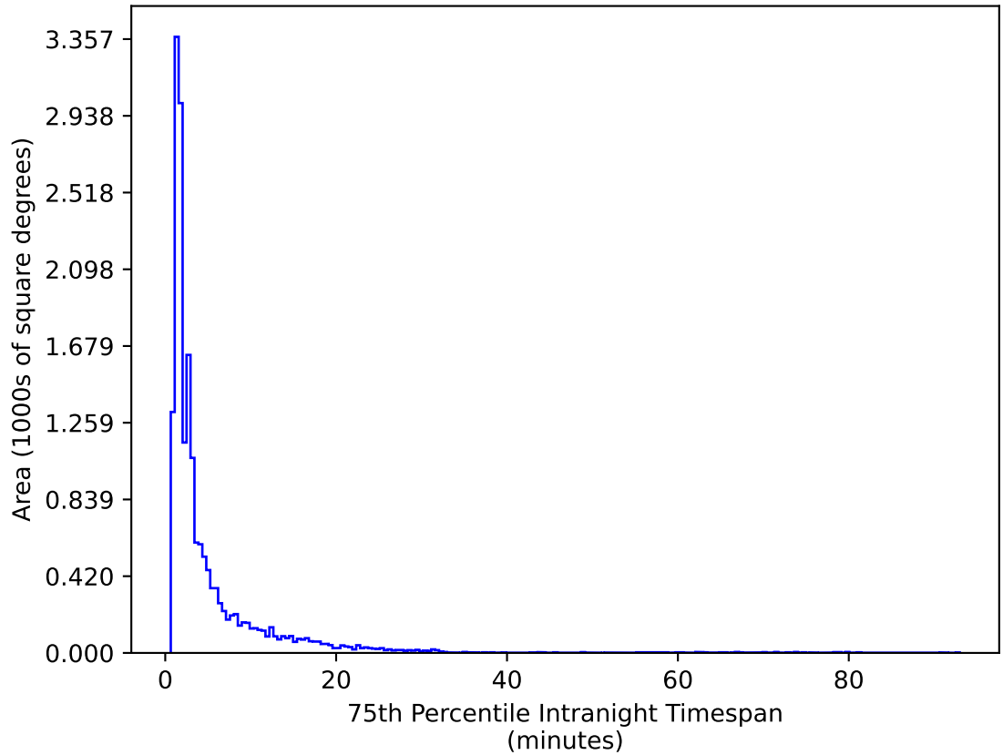
ddf_loaded_fl4_v3.4_10yrs WFD g band: 75th Percentile Intranight Timespan
