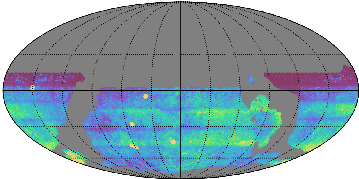
ddf_loaded_fl4_v3.4_10yrs WFD all bands: 75th Percentile Intranight Timespan
