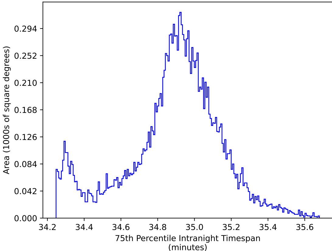
ddf_loaded_fl4_v3.4_10yrs WFD all bands: 75th Percentile Intranight Timespan
