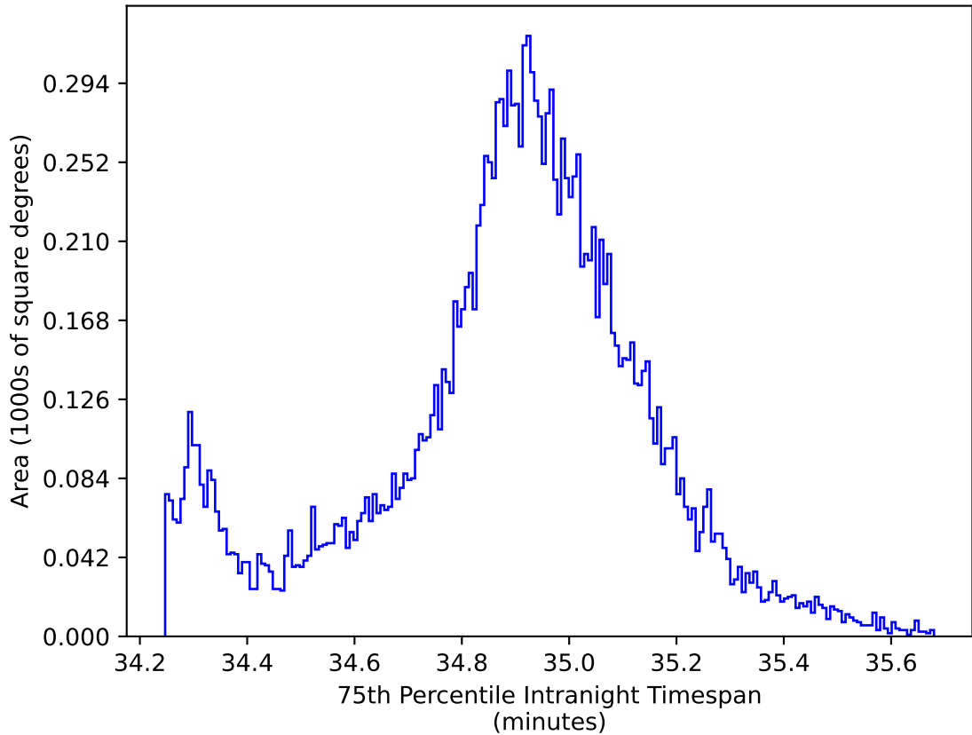
ddf_loaded_fl4_v3.4_10yrs WFD: 75th Percentile Intranight Timespan
