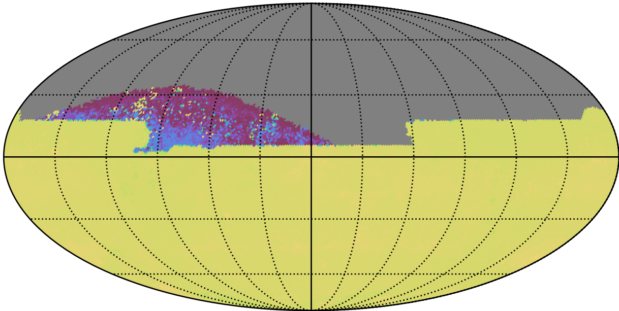
ddf_loaded_fl4_v3.4_10yrs All sky zy bands: 75th Percentile Intranight Timespan
