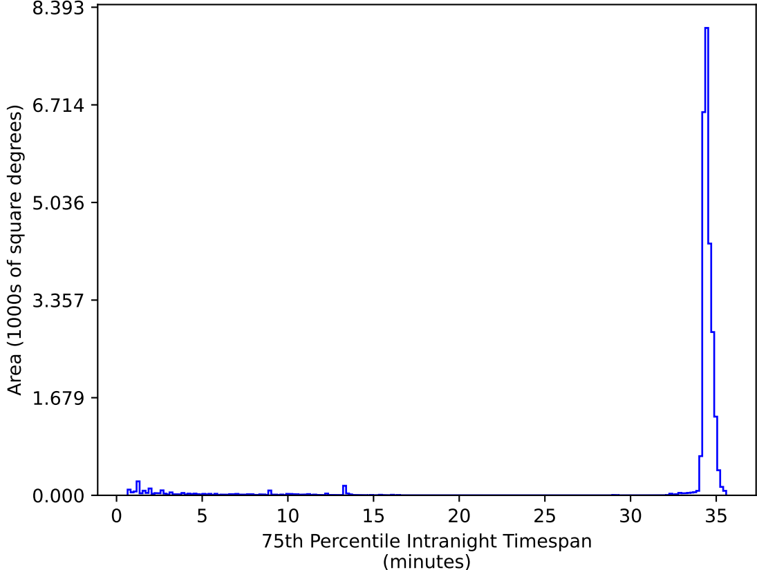
ddf_loaded_fl4_v3.4_10yrs All sky zy bands: 75th Percentile Intranight Timespan
