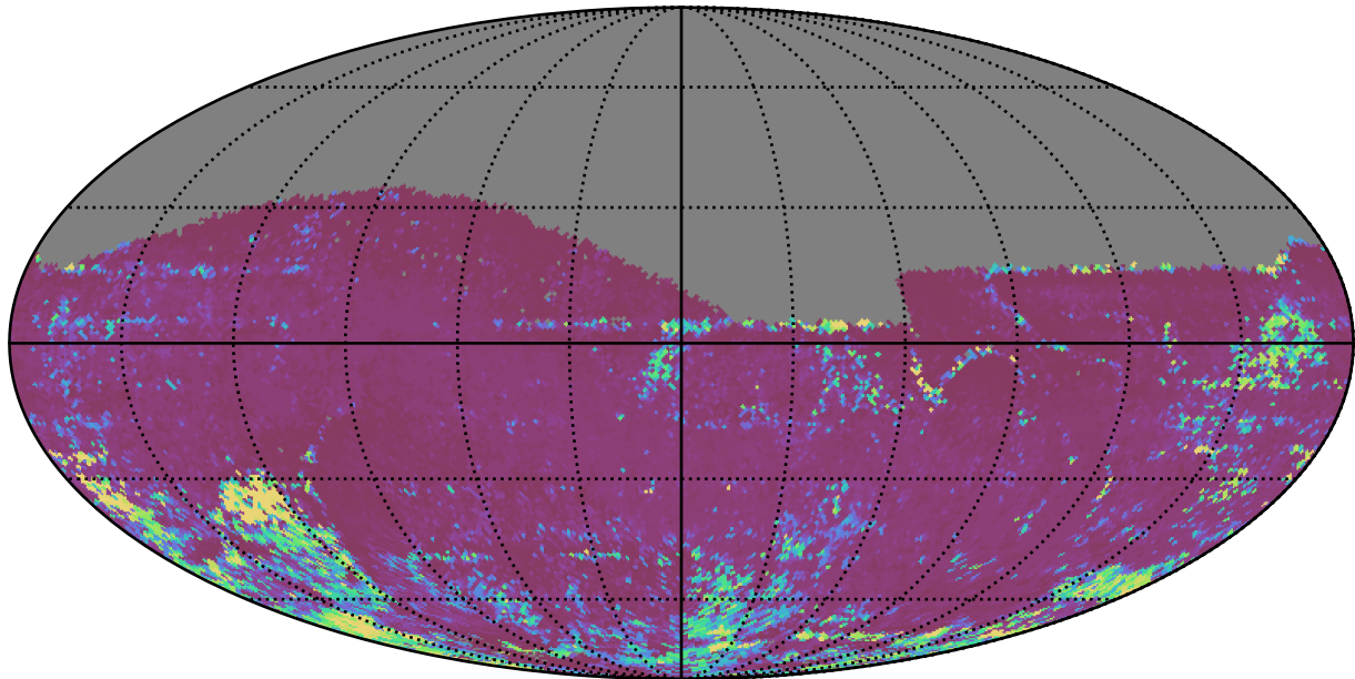
ddf_loaded_fl4_v3.4_10yrs All sky z band: 75th Percentile Intranight Timespan
