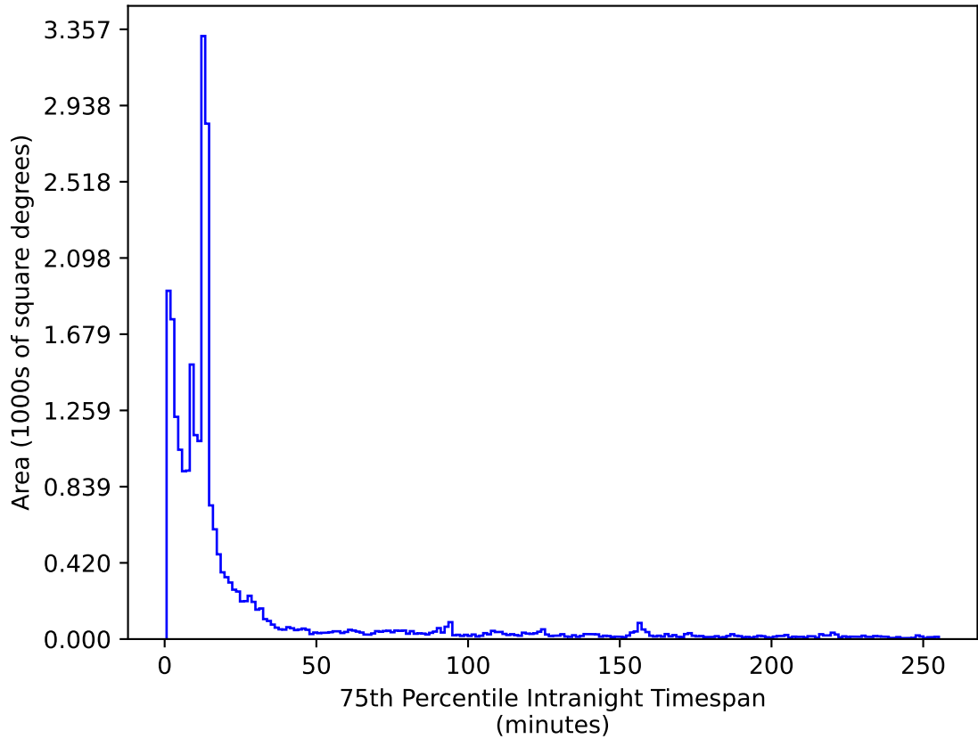
ddf_loaded_fl4_v3.4_10yrs All sky z band: 75th Percentile Intranight Timespan
