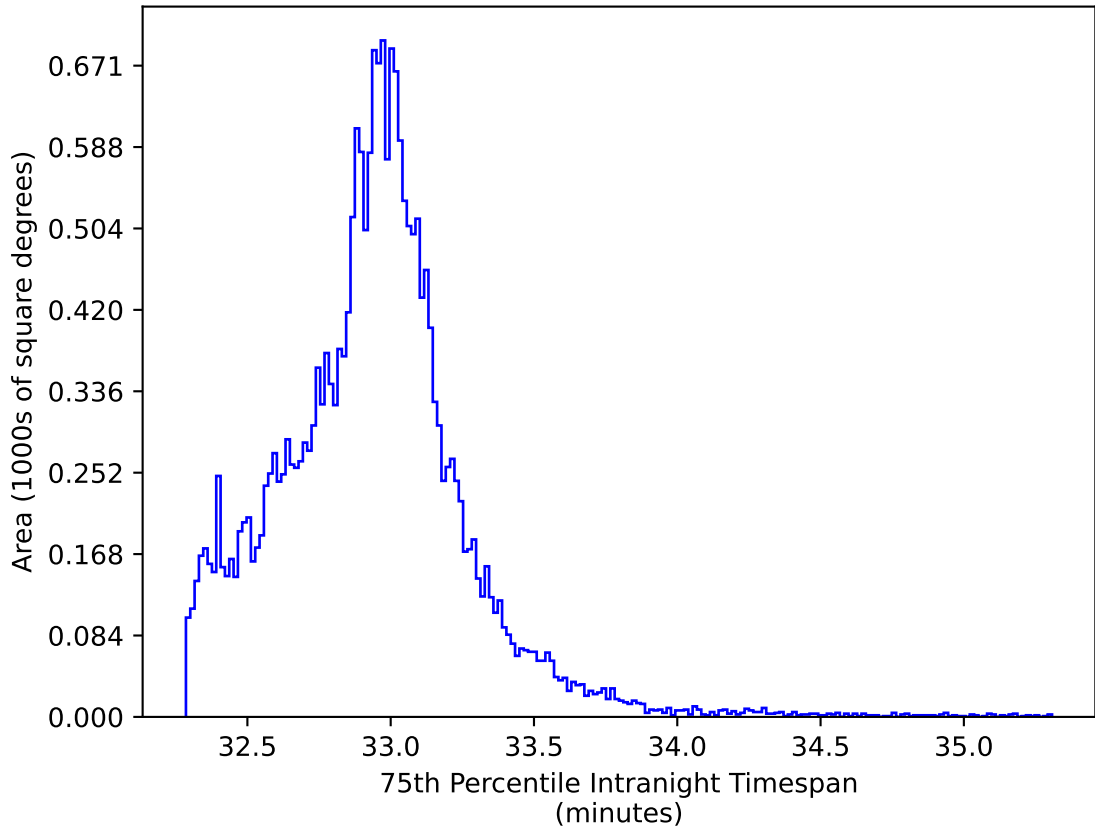
ddf_loaded_fl4_v3.4_10yrs All sky y band: 75th Percentile Intranight Timespan
