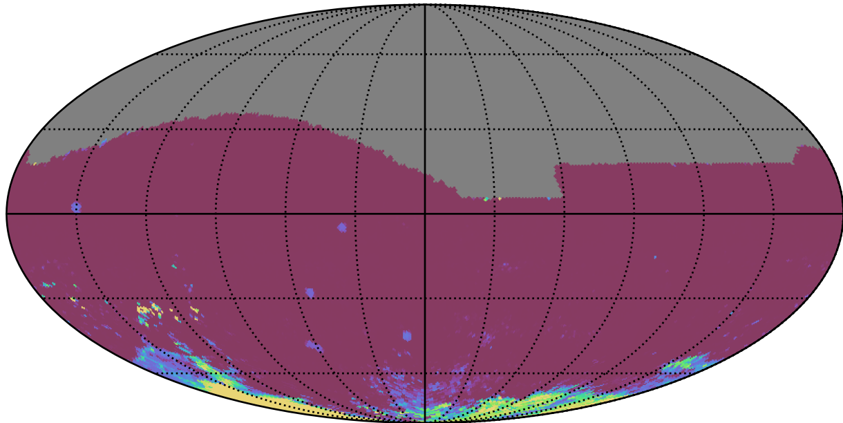
ddf_loaded_fl4_v3.4_10yrs All sky ri bands: 75th Percentile Intranight Timespan
