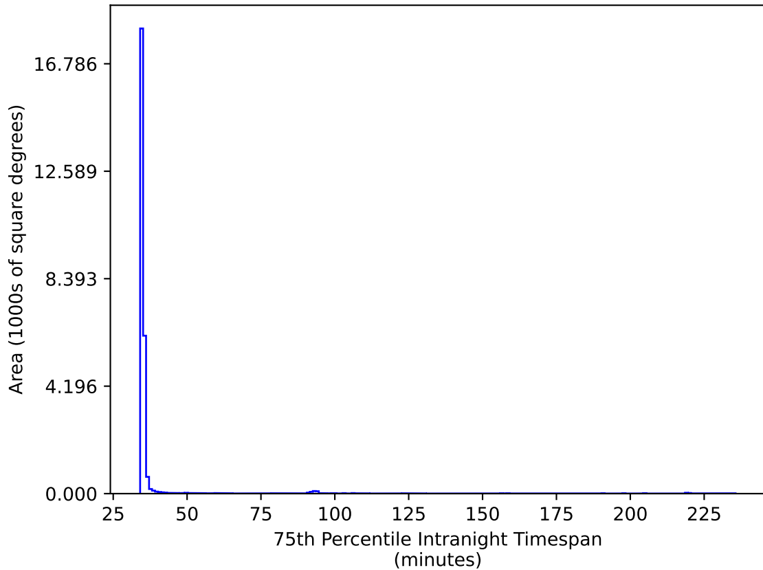
ddf_loaded_fl4_v3.4_10yrs All sky ri bands: 75th Percentile Intranight Timespan
