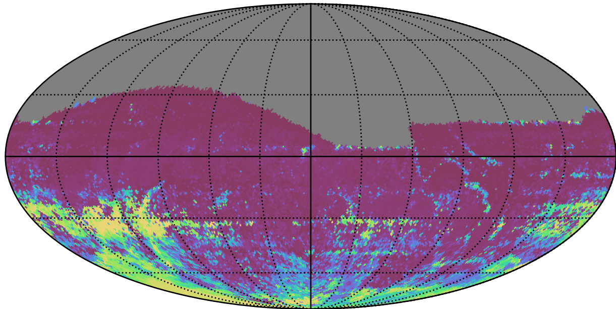
ddf_loaded_fl4_v3.4_10yrs All sky r band: 75th Percentile Intranight Timespan
