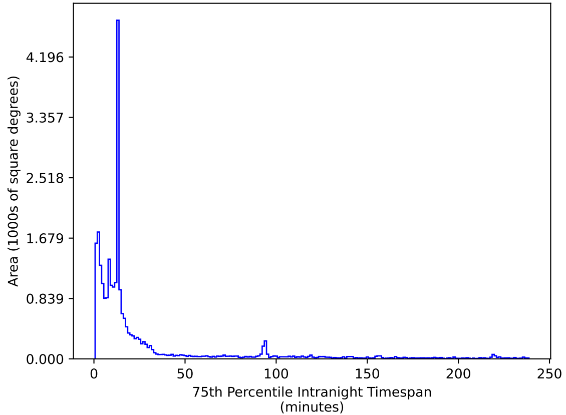
ddf_loaded_fl4_v3.4_10yrs All sky i band: 75th Percentile Intranight Timespan
