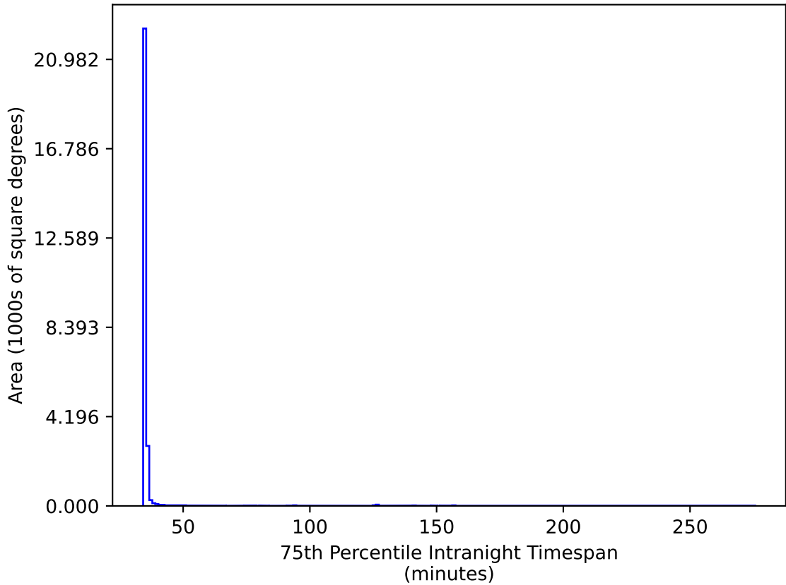
ddf_loaded_fl4_v3.4_10yrs All sky gr bands: 75th Percentile Intranight Timespan
