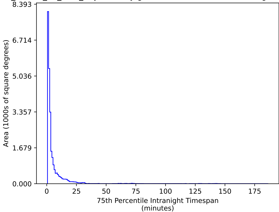
ddf_loaded_fl4_v3.4_10yrs All sky g band: 75th Percentile Intranight Timespan
