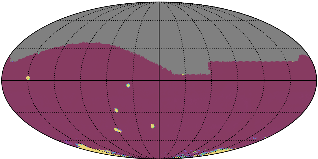
ddf_loaded_fl4_v3.4_10yrs All sky all bands: 75th Percentile Intranight Timespan
