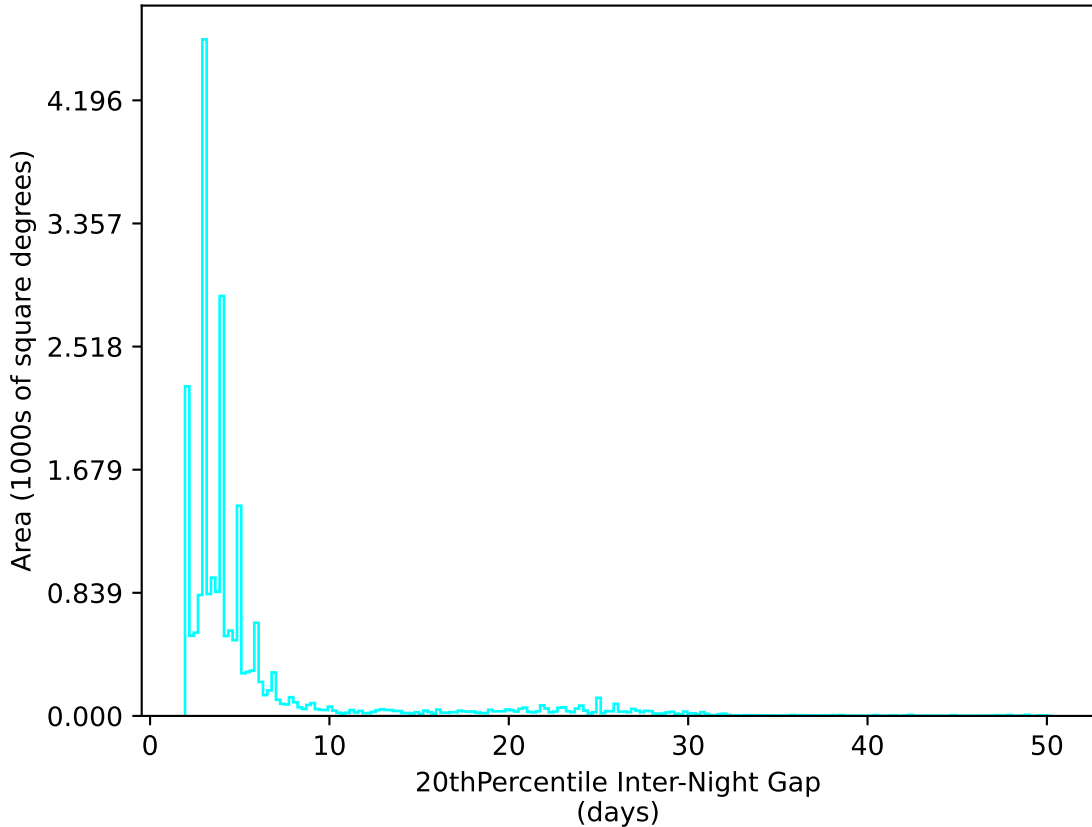
ddf_loaded_fl4_v3.4_10yrs All sky u band: 20thPercentile Inter-Night Gap
