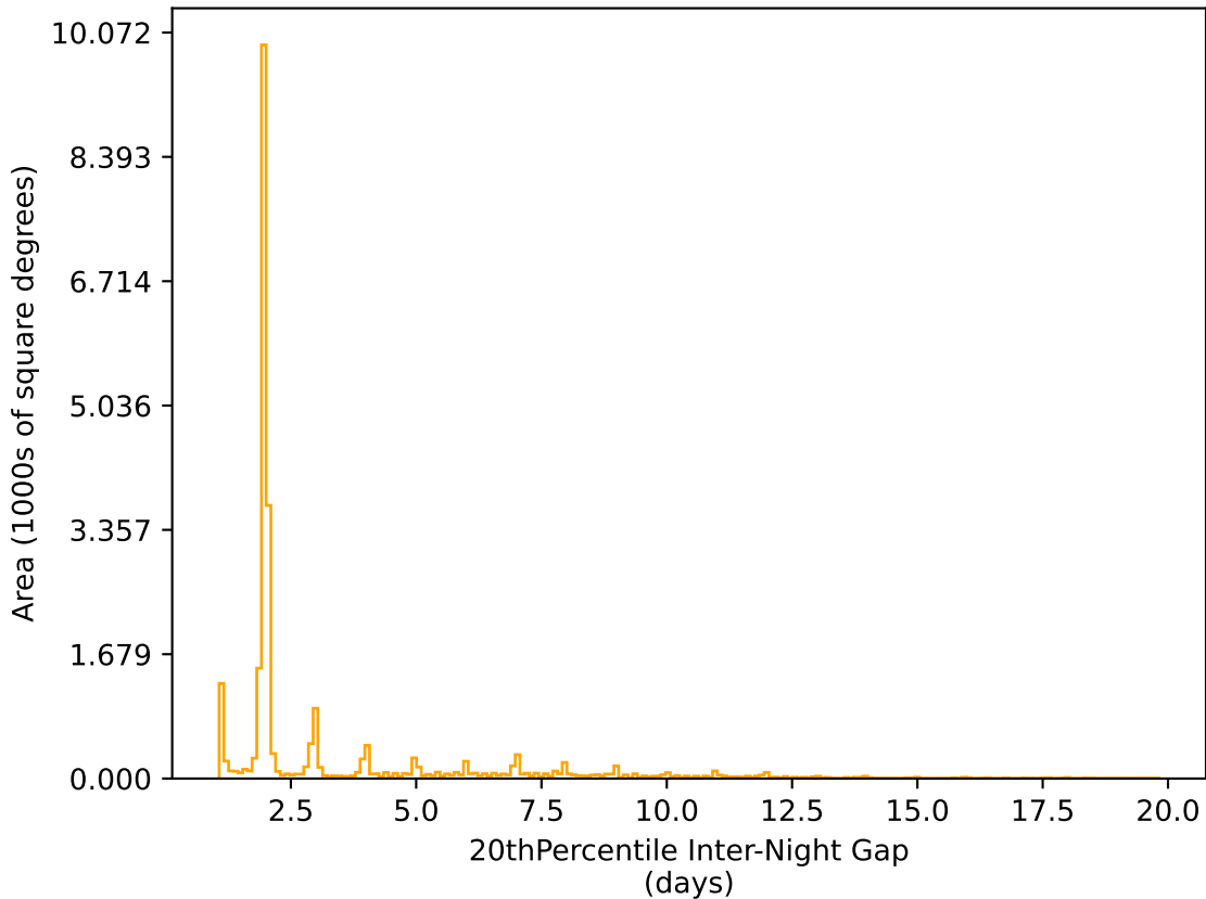
ddf_loaded_fl4_v3.4_10yrs All sky r band: 20thPercentile Inter-Night Gap
