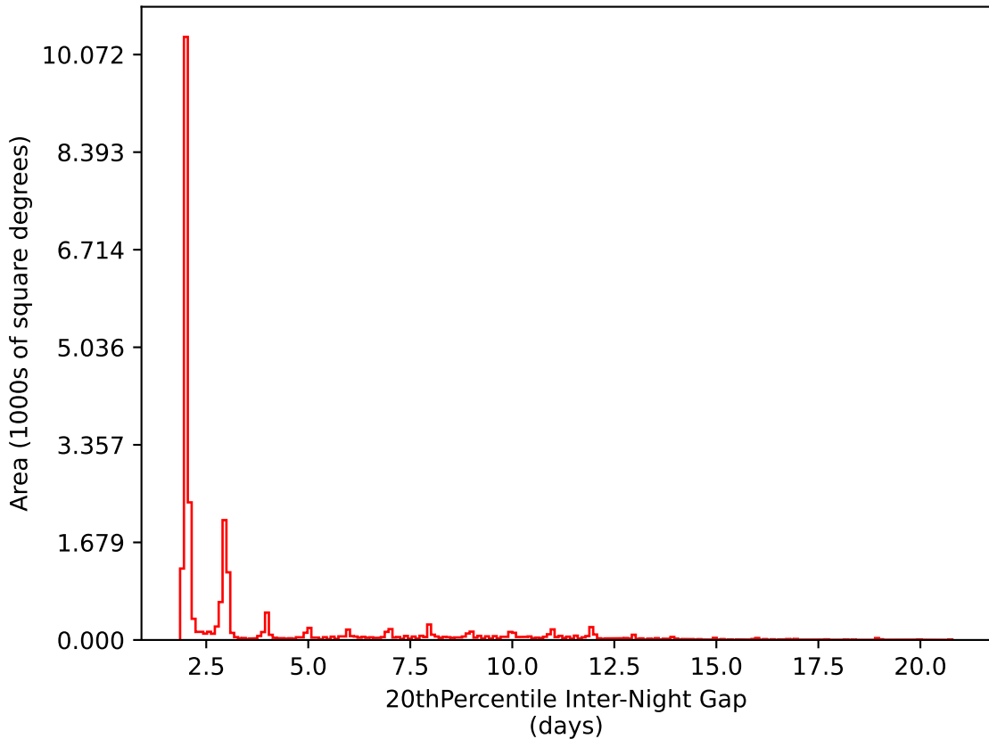
ddf_loaded_fl4_v3.4_10yrs All sky i band: 20thPercentile Inter-Night Gap
