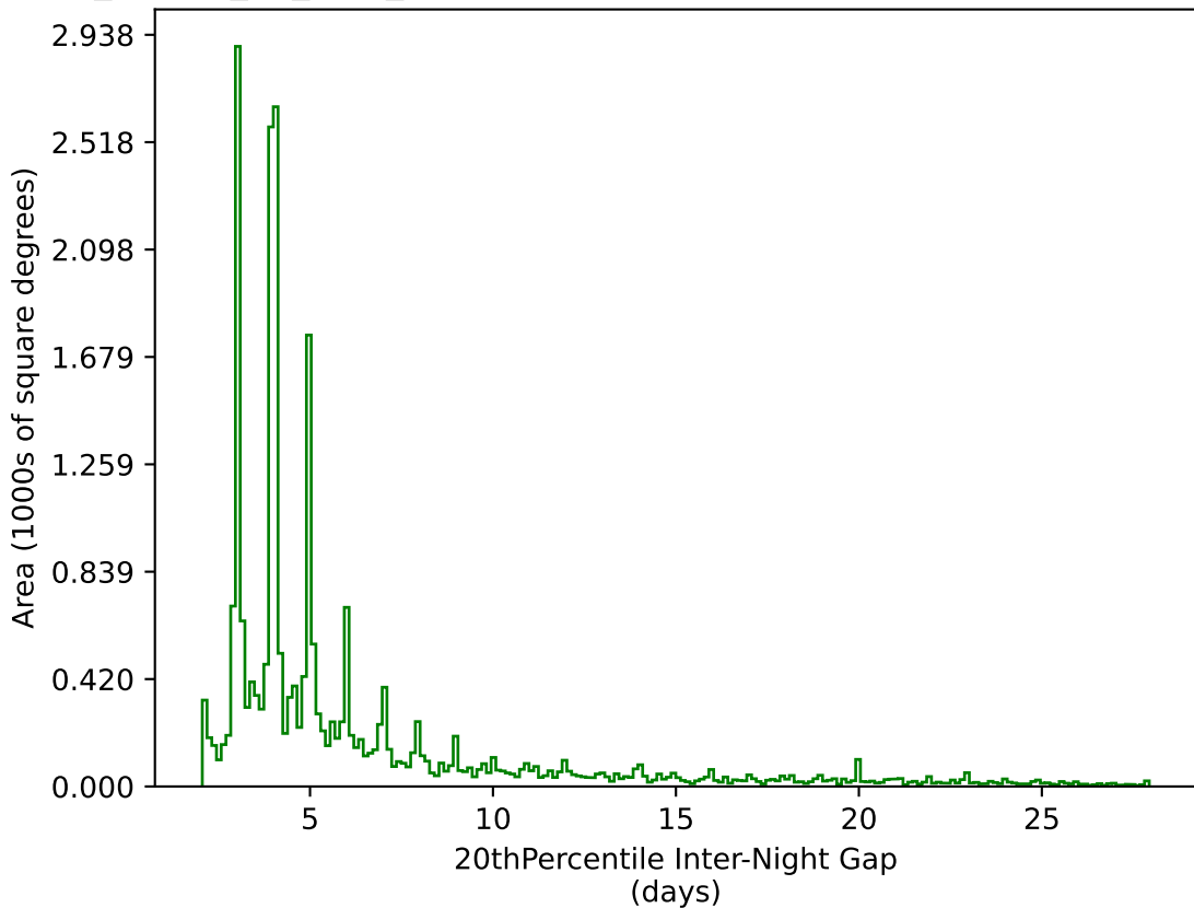
ddf_loaded_fl4_v3.4_10yrs All sky g band: 20thPercentile Inter-Night Gap
