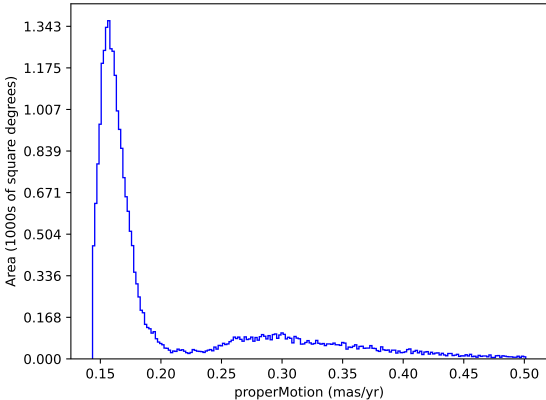
ddf_loaded_fl4_v3.4_10yrs : properMotion
