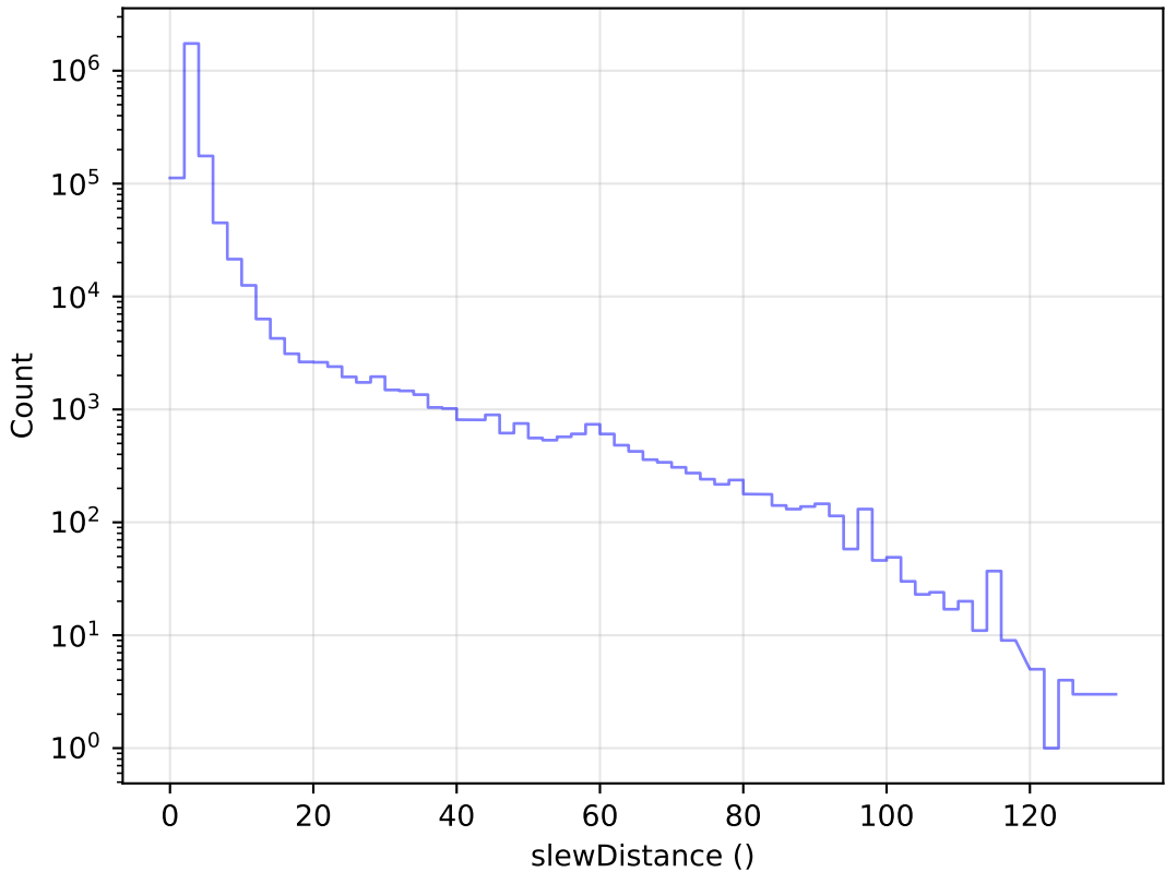
ddf_loaded_fl4_v3.4_10yrs All visits: Slew Distance Histogram
