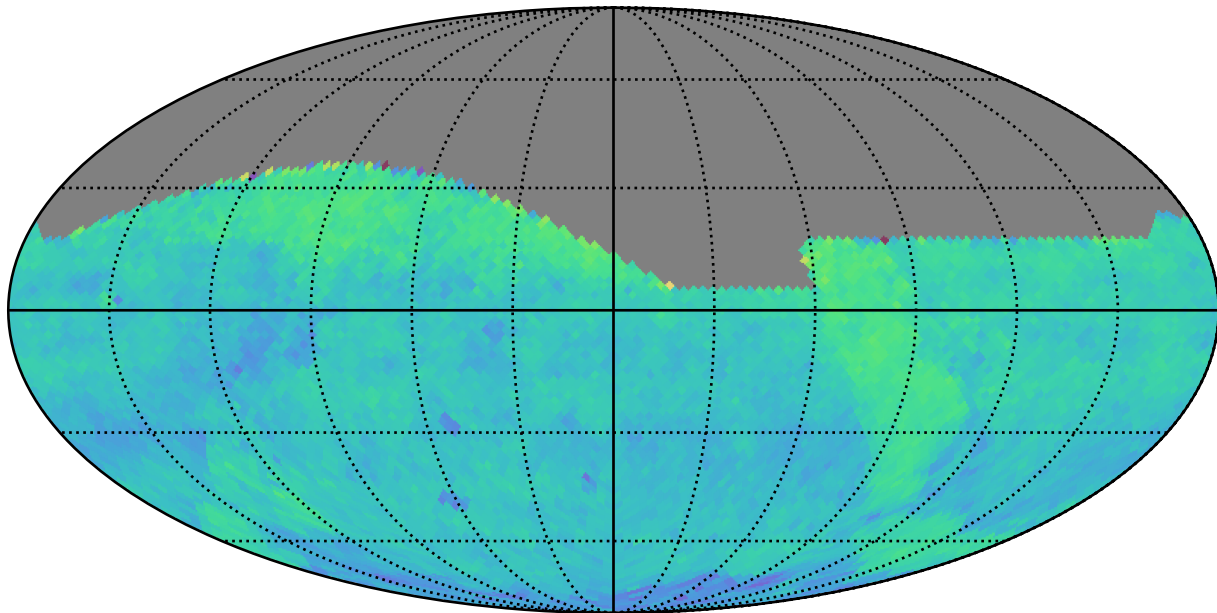
ddf_loaded_fl4_v3.4_10yrs (g or r or i): PairFraction
