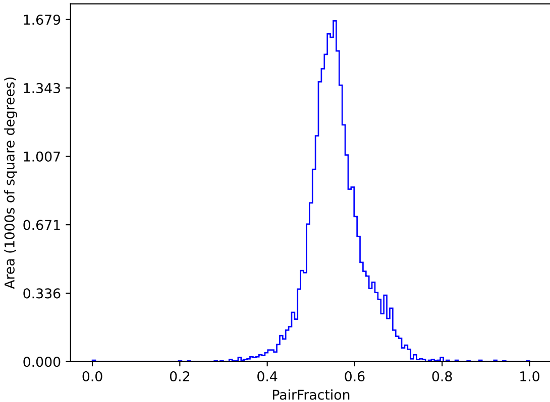
ddf_loaded_fl4_v3.4_10yrs (g or r or i): PairFraction
