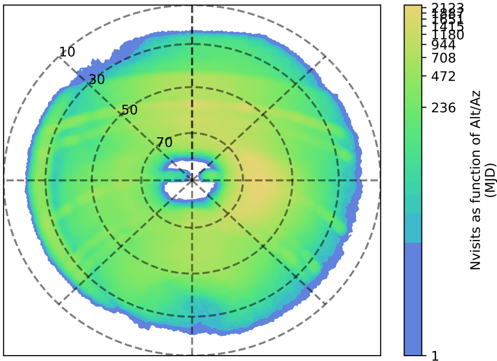
ddf_loaded_fl4_v3.4_10yrs r: Nvisits as function of Alt/Az
