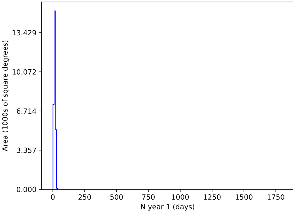
ddf_loaded_fl4_v3.4_10yrs z and night < 365: N year 1
