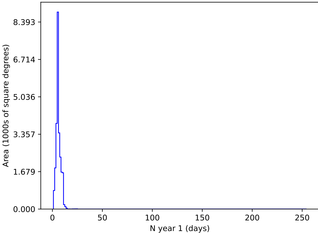
ddf_loaded_fl4_v3.4_10yrs u and night < 365: N year 1
