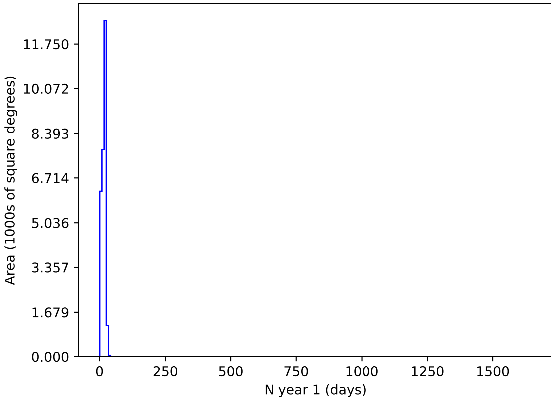
ddf_loaded_fl4_v3.4_10yrs r and night < 365: N year 1
