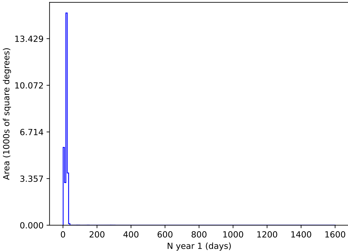
ddf_loaded_fl4_v3.4_10yrs i and night < 365: N year 1
